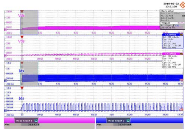
Figure 52 – 115 VAC Input.
