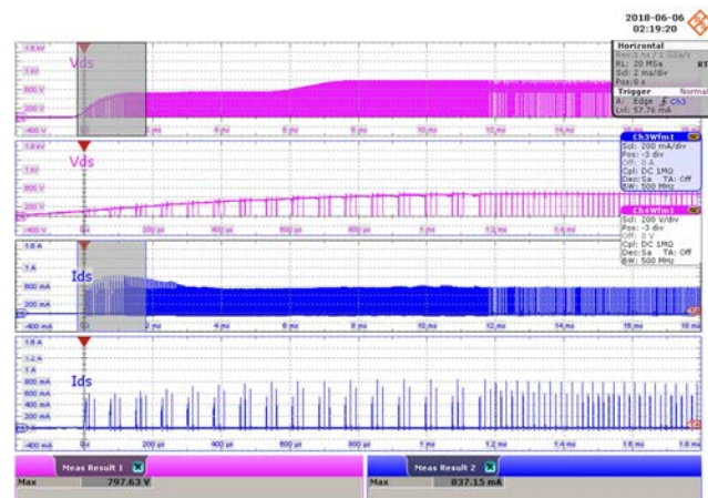
Figure 54 – 450 VAC Input.
