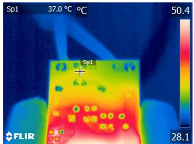
Figure 82 – Ambient = 28.1 °C. Bridge Rectifier, BR1 = 37.0 °C.
