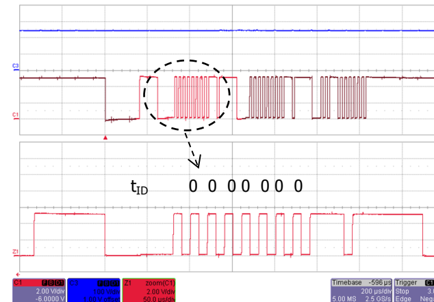
Figure 40 – Status Query - Device ID 3 Response, Phase W. Status Update: 000 00 0 0 (clear) Upper: V_{BUS} , 100 V / div. Lower: V_{FAULT} , 2 V / div., 200 \mu s / div. Zoom: 50 \mu s / div.
