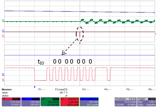
Figure 34 – Bus Sensing - OV Threshold Cleared. Bus Voltage Drop 430 to 340 VDC. Status Update: 000 00 0 0 (OV Cleared). Upper: V_{BUS} , 100 V / div. Middle: I_{PHASE U} , 500 mA / div. Lower: V_{FAULT} , 2 / div., 10 ms / div. Zoom: 50 \mu s / div.
