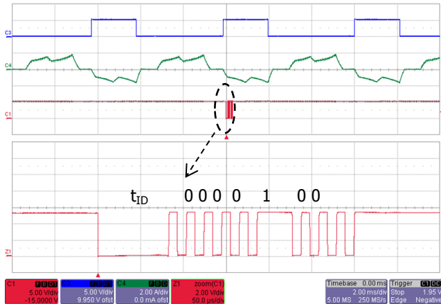
Figure 23 – Temperature Warning, Phase W. Status Update: 000 01 0 0 (OTW). Upper: INL Input, 5 V / div. Middle: I_{PHASE W} , 2 A / div. Lower: V_{FAULT} , 2 V / div., 2 ms / div. Zoom: 50 \mu s / div.
