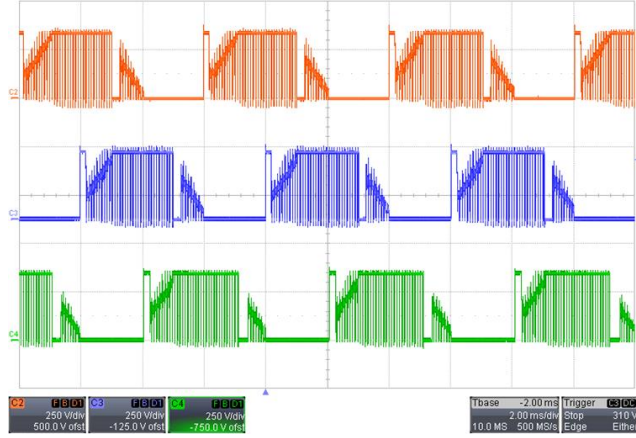
Figure 7 – Steady-State – 5000 RPM, Full Load. Upper: V_{HB(PHASE U)} , 250 V / div. Middle: V_{HB(PHASE V)} , 250 V / div. Lower: V_{HB(PHASE W)} , 250 V / div. Time Scale: 2 ms / div.
