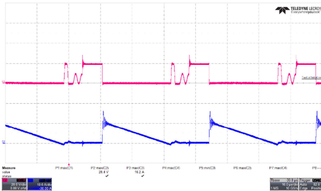
Figure 78 – SR FET Voltage Waveforms. 90 VAC, 5.0 V, 3 A Load (28.4 V MAX ). Upper: V DRAIN , 20 V / div. Lower: I DRAIN , 10 A / div. Time: 10 μs / div.
