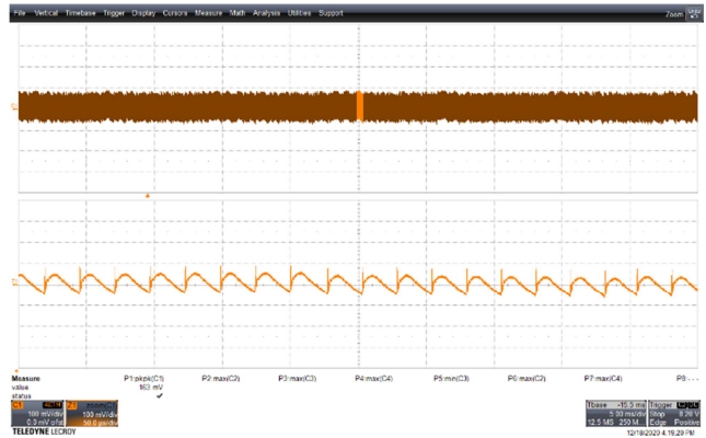
Figure 101 – Output Ripple. PK-PK = 163 mV 115 V ACIN 9.0 V, 3 A Load. V OUT , 100 mV / div., 5 ms / div. Zoom: 50 μs / div.
