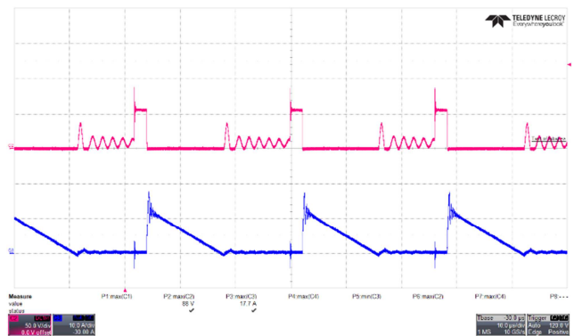
Figure 81 – SR FET Voltage Waveforms. 265 VAC, 9.0 V, 3 A Load (88 V MAX ). Upper: V DRAIN , 50 V / div. Lower: I DRAIN , 10 A / div. Time: 10 μs / div.
