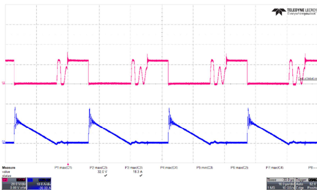
Figure 80 – SR FET Voltage Waveforms. 90 VAC, 9.0 V, 3 A Load (32.0 V MAX ). Upper: V DRAIN , 20 V / div. Lower: I DRAIN , 10 A / div. Time: 10 μs / div.
