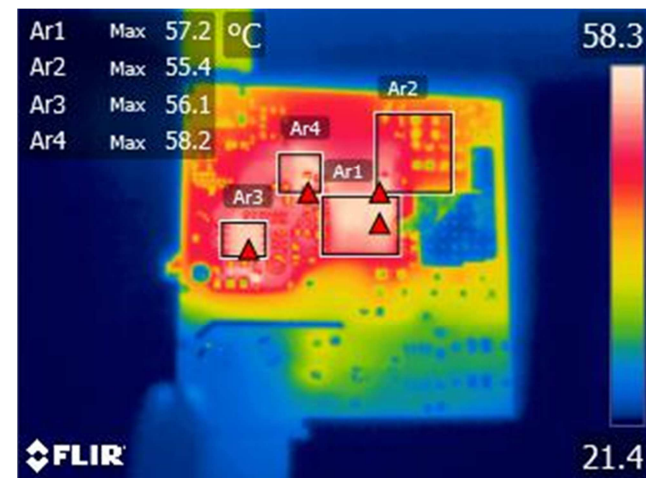
Figure 29 – Bottom Thermal Image.
