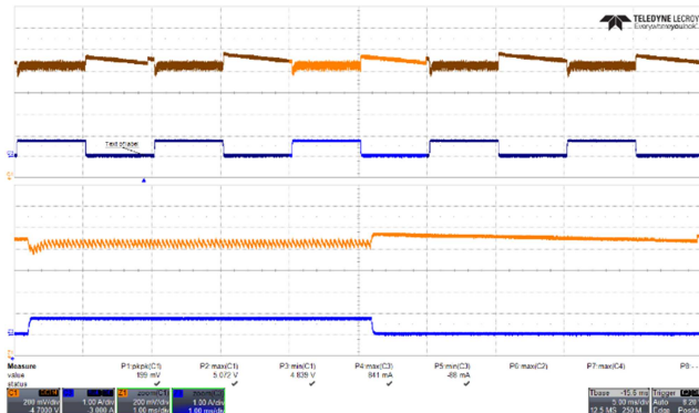
Figure 38 – Transient Response. 90 VAC, 5.0 V, 0 – 0.75 A Load Step. V_{MIN} : 4.839 V, V_{MAX} : 5.072 V. Upper: V_{OUT} , 0.2 V / div., 5 ms / div. Lower: I_{LOAD} , 1 A / div. Zoom: 1 ms / div.
